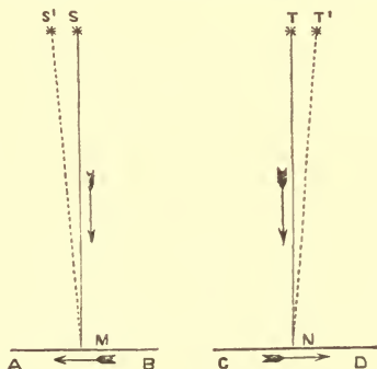
Aberration of Light.
